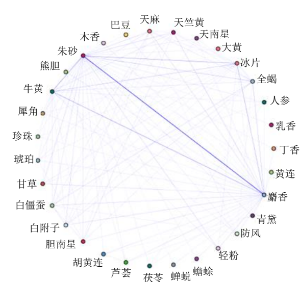
图 5 含雄黄儿科方剂配伍核心药物网络 Fig. 5 Core drug network diagram of pediatric prescription containing realgar
