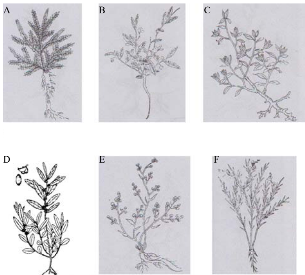
A-《图经》解州远志 B-《图考》瓜子金 C-《图经》泗州远志 D-《中华本草》华南远志 E-《图经》商州远志 F-《救荒》远志 A- P. tenuifolia in Bencao Tujing B- P. japonica in Textual Research on Reality and Titles of Plants C- P. glomerata in Bencao Tujing D- P. glomerata in Chinese Materia Medica E- P. crotalarioides in Bencao Tujing F- P. tenuifolia in Herbal for Relief of Famines
