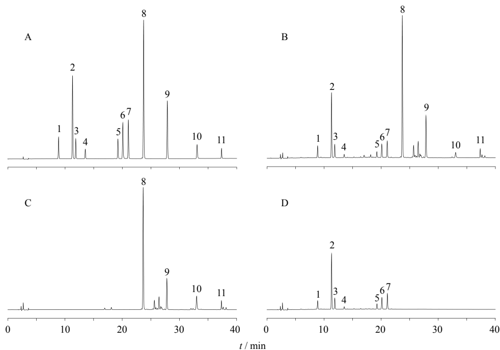
1-新绿原酸 2-绿原酸 3-隐绿原酸 4-咖啡酸 5-异绿原酸 B 6-异绿原酸 A 7-异绿原酸 C 8-黄芩苷 9-汉黄芩苷 10-黄芩素 11-汉黄芩素 1-neochlorogenic acid 2-chlorogenic acid 3-cryptochlorogenic acid 4-cafferic acid 5-isochlorogenic acid B 6-isochlorogenic acid A 7-isochlorogenic acid C 8-baicalin 9-wogonoside 10-baicalein 11-wogonin
