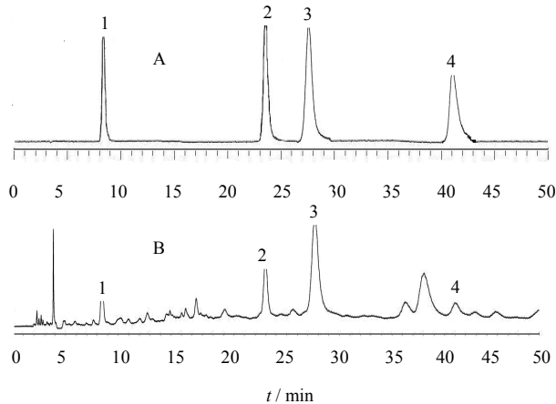
1-没食子酸 2-柯里拉京 3-老鹳草素 4-短叶苏木酚酸 1-gallic acid 2-corilagin 3-geraniin 4-brevifolin carboxylic acid
