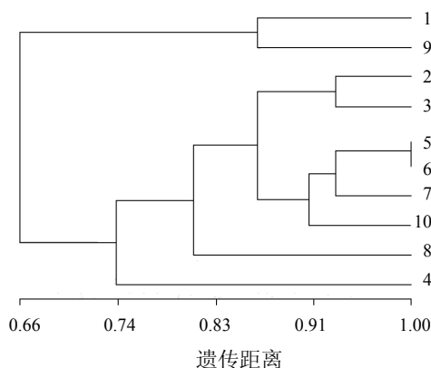
图 5 10 个不同产地白头翁 UPGMA 聚类结果 Fig. 5 UPGMA cluster analysis on P. chinensis from ten different habitats
