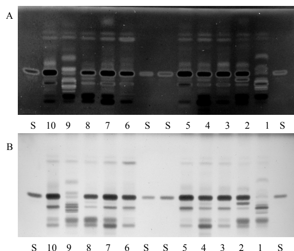
图 4 366 nm (A) 和白光 (B) 下白头翁高效薄层色谱图 Fig. 4 HPTLC chromatograms of P. chinensis at 366 nm (A) and under white light (B)
