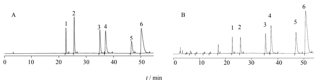
1-盐酸药根碱 2-盐酸非洲防己碱 3-盐酸表小檗碱 4-盐酸黄连碱 5-盐酸巴马汀 6-盐酸小檗碱 1-jatrorhizine hydrochloride 2-columbamine hydrochloride 3-epiberberine hydrochloride 4-coptisine hydrochloride 5-palmatine hydrochloride 6-berberine hydrochloride
