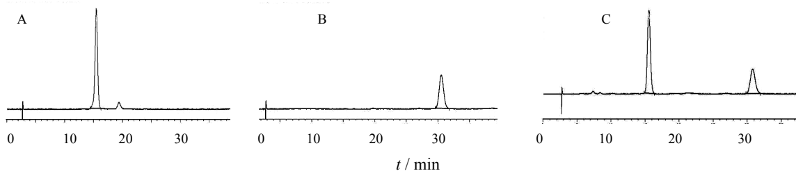
图 2 西红花苷-I (A)、西红花苷-II (B)、西红花样品 (C) 的色谱图 Fig.2 Chromatograms of crocin-I (A), crocin-II (B), and saffron samples (C)
