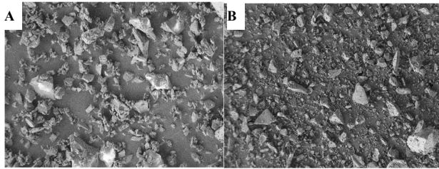
图1 普通白藜芦醇(A)和纳米级白藜芦醇(B)电镜图 Fig. 1 Electron micrograph of common (A) and nanometer (B) preparation of resveratrol
