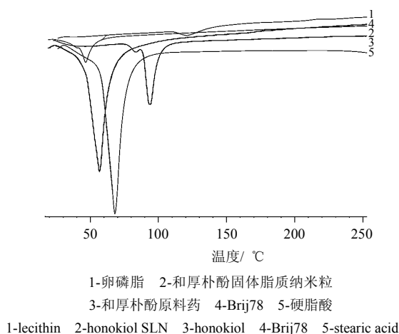
图2 和厚朴酚及其制剂和辅料的差示扫描量热图谱 Fig. 2 DSC Curves of honokiol, its preparations and accessories
