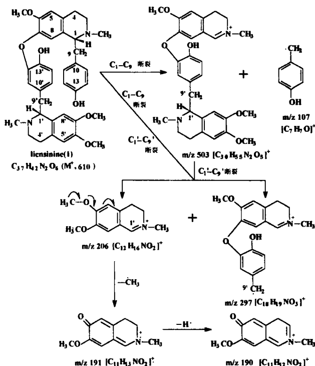
Fig. 1 Major Fragments of Liensinine
