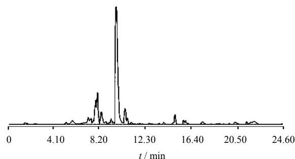
图1 \text{ESI}^+ 模式下对照组大鼠尿液典型总离子流图 Fig. 1 Typical TIC chromatogram of urine in rats of control group under \text{ESI}^+ mode
